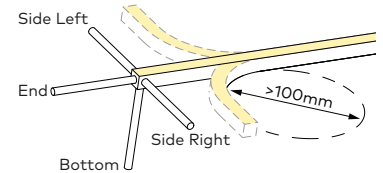
Horizontal Bending
